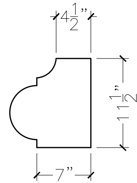
SECTION VIEW
