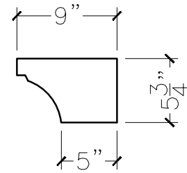
SECTION VIEW
