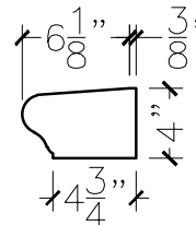
SECTION VIEW
