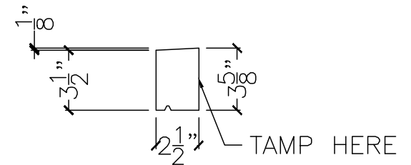
SECTION VIEW
