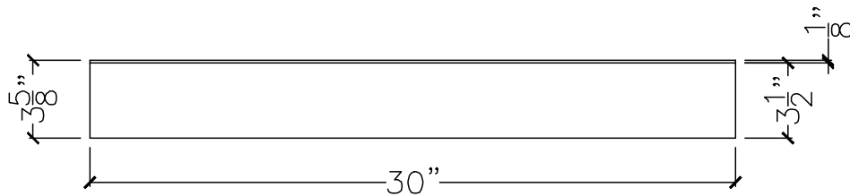
FRONT VIEW
