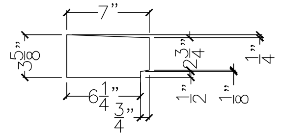
SECTION VIEW
