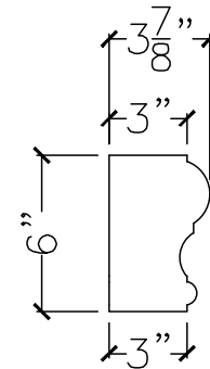
SECTION VIEW
