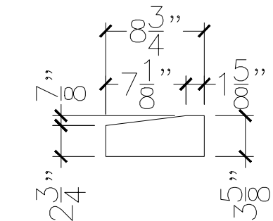
SECTION VIEW
