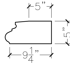
SECTION VIEW
