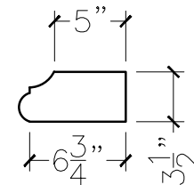
SECTION VIEW
