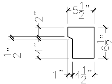
SECTION VIEW
