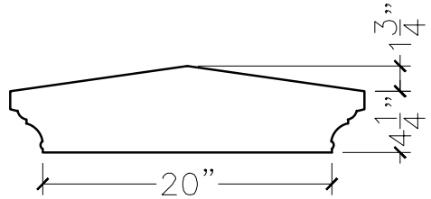
SECTION VIEW
