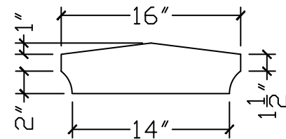
SECTION VIEW
