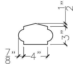
SECTION VIEW
