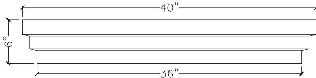
FRONT VIEW
