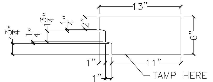
SECTION VIEW
