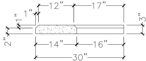
SECTION VIEW
