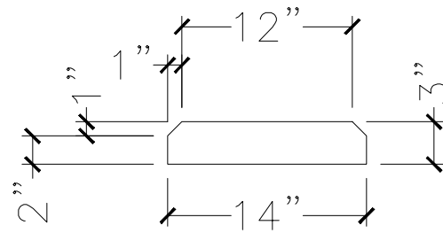
SECTION VIEW
