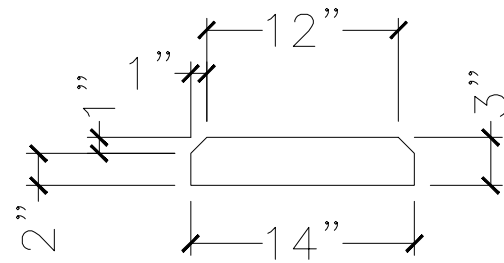
SECTION VIEW
