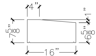
SECTION VIEW
