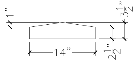
SECTION VIEW
