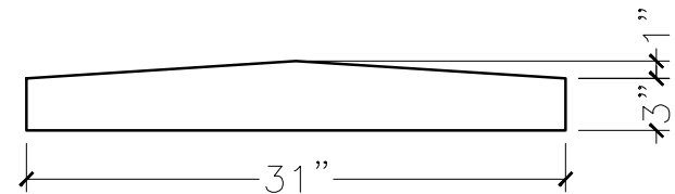
SECTION VIEW
