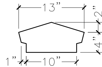
SECTION VIEW
