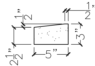
SECTION VIEW
