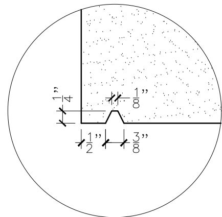
*DRIP DETAIL*
