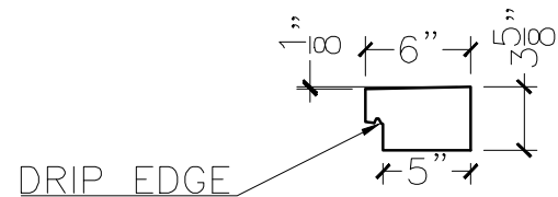
SECTION VIEW
