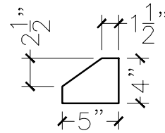
SECTION VIEW
