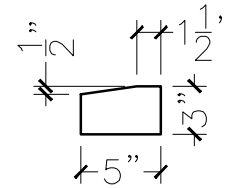
SECTION VIEW
