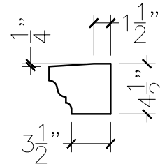
SECTION VIEW
