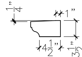
SECTION VIEW
