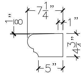
SECTION VIEW
