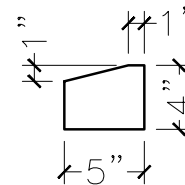
SECTION VIEW
