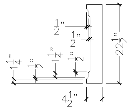
SECTION VIEW
