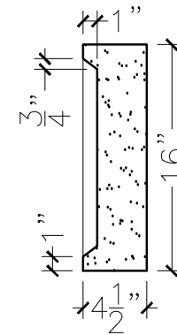
SECTION VIEW
