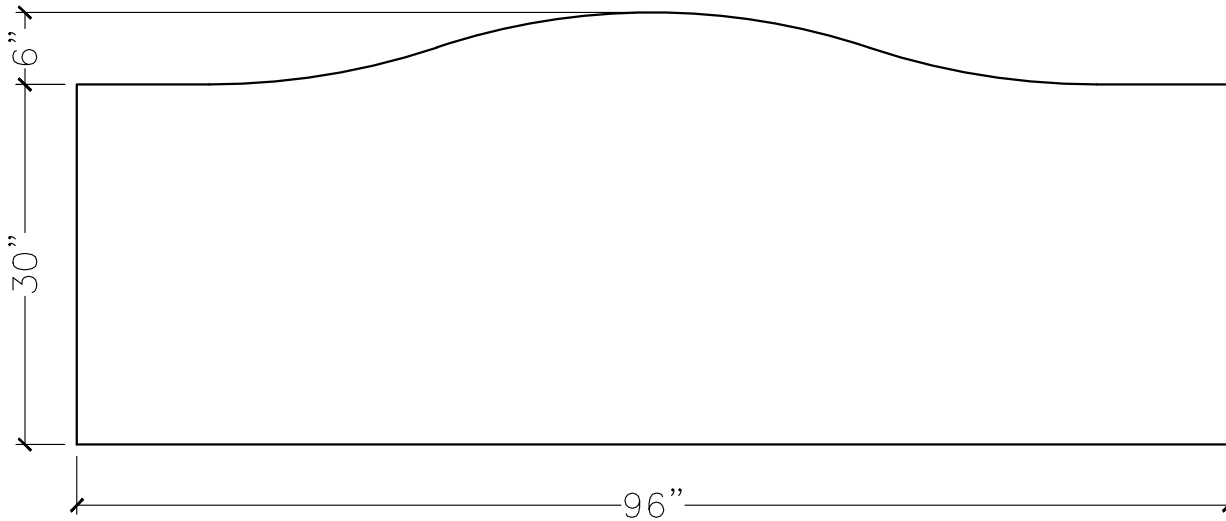
FRONT VIEW
