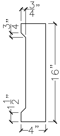
SECTION VIEW
