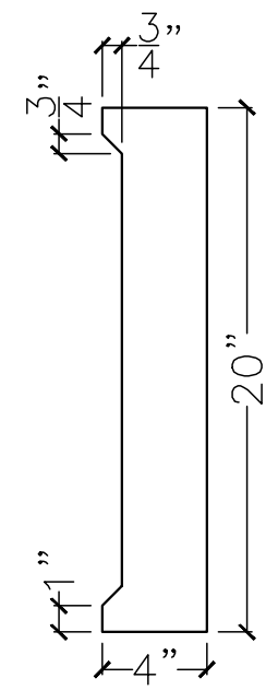
SECTION VIEW
