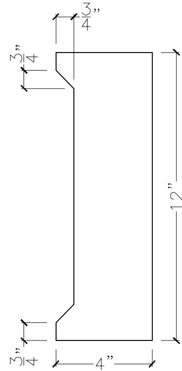
SECTION VIEW
