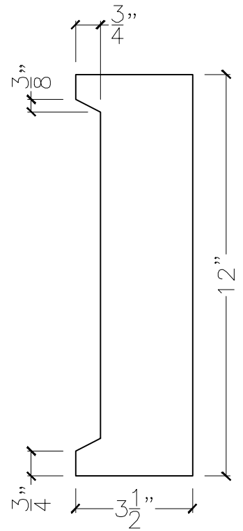
SECTION VIEW
