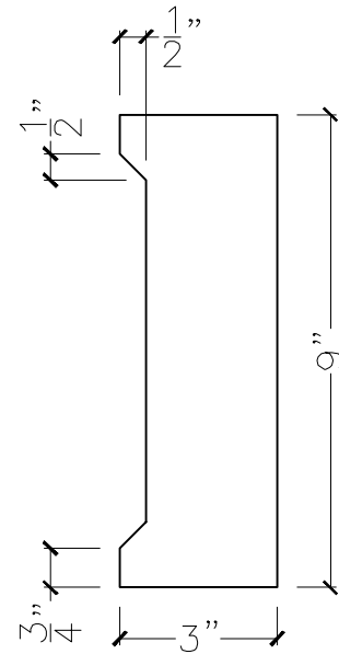
SECTION VIEW
