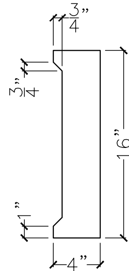
SECTION VIEW
