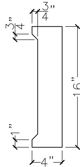
SECTION VIEW
