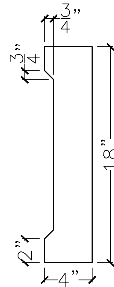
SECTION VIEW
