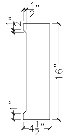
SECTION VIEW
