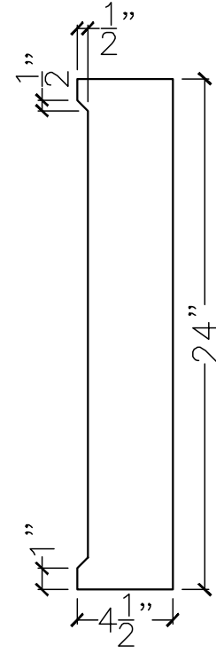
SECTION VIEW
