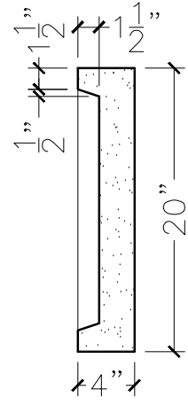
SECTION VIEW
