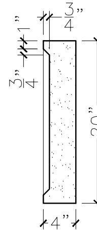
SECTION VIEW
