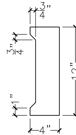
SECTION VIEW
