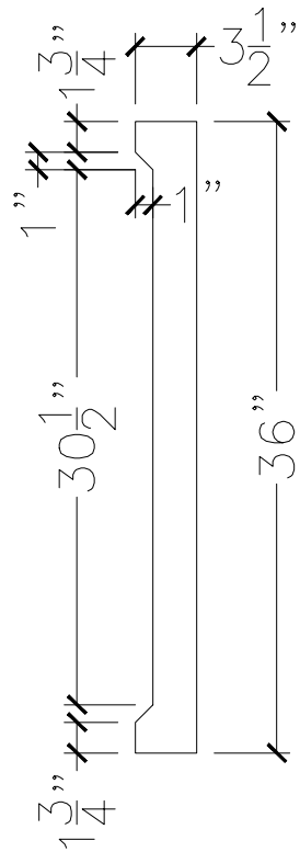
SECTION VIEW
