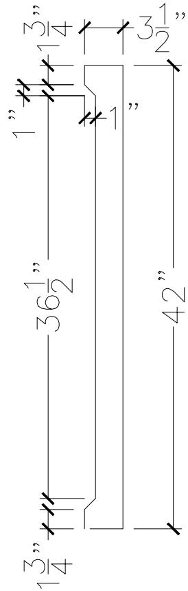
SECTION VIEW
