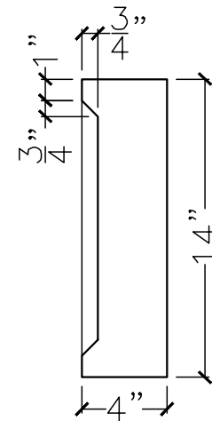
SECTION VIEW
